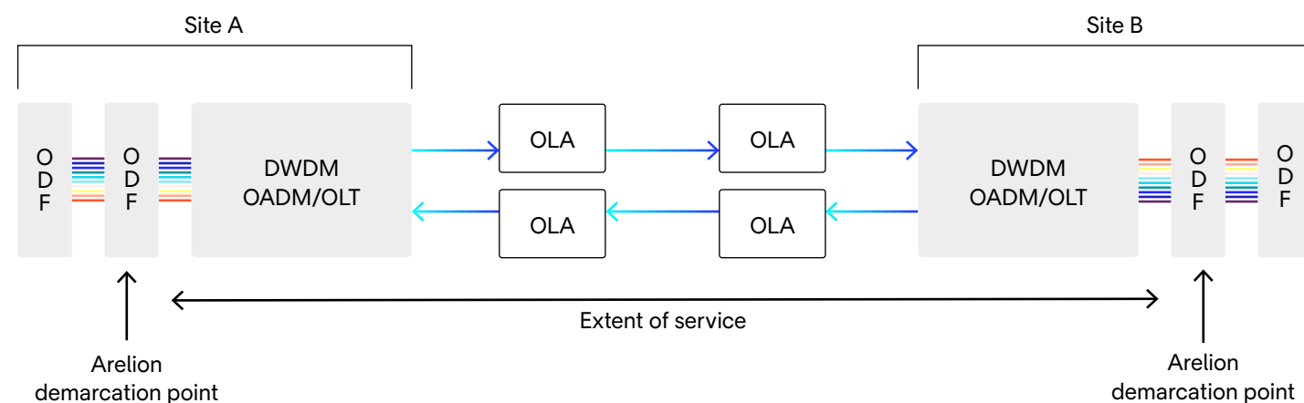
DWDM network components
